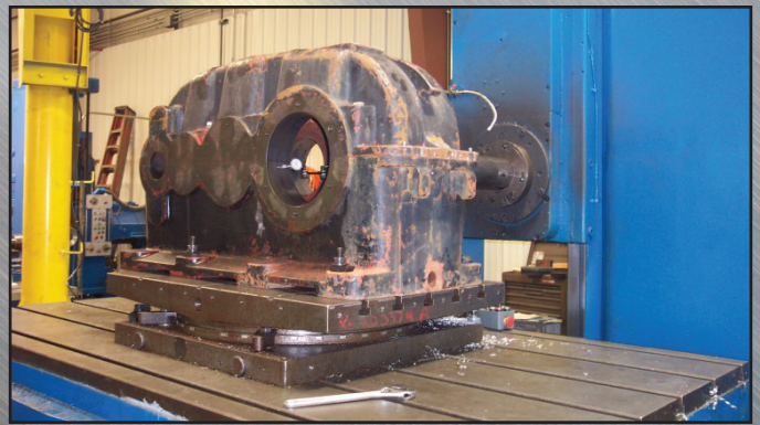
Oil Field Casting - Repaired and Line Bored
